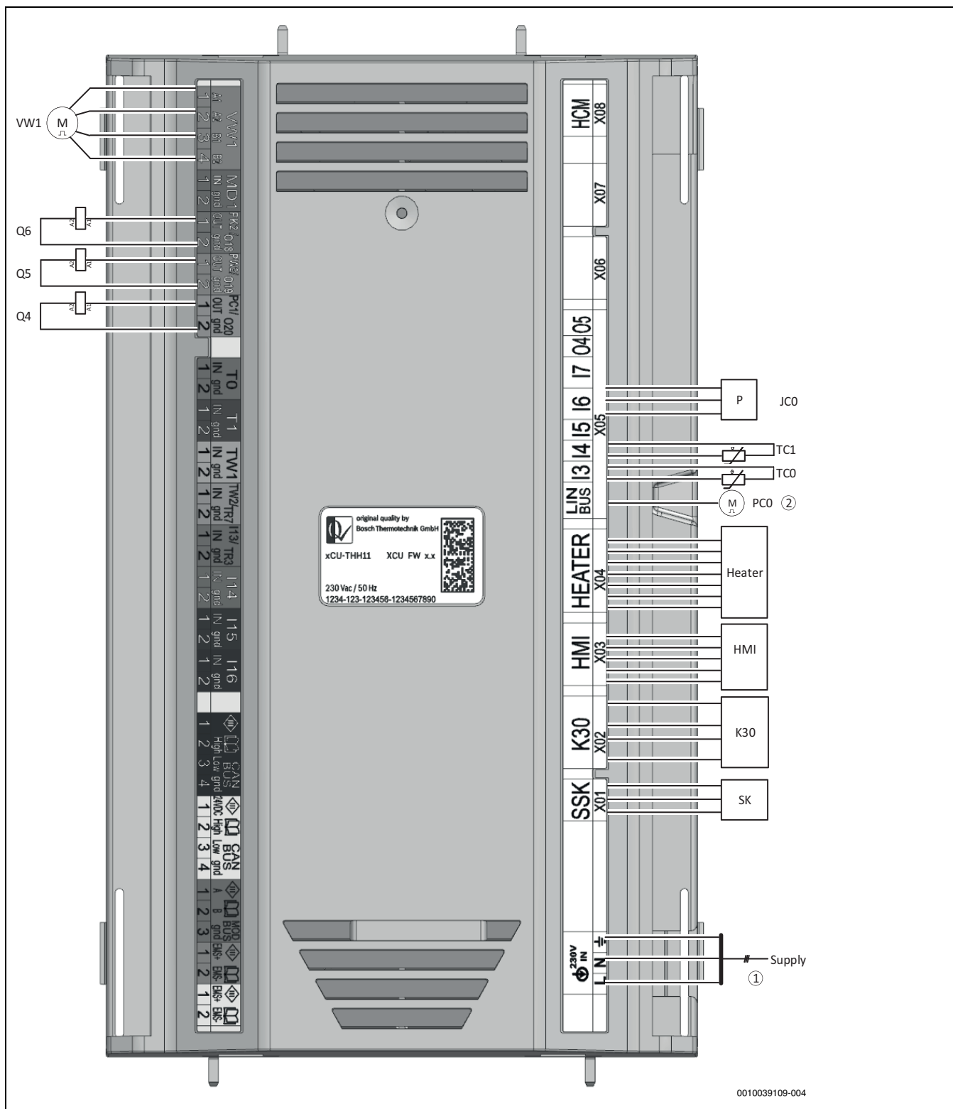
Afb. 41 Schakelschema XCU-THH (XCU HY)
