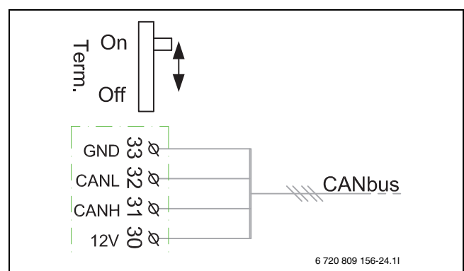
Afb. 10 CAN-BUS-beëindiging
