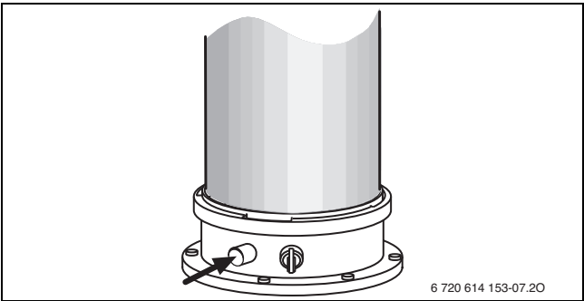
Afb. 39 Rookgasmeetnippel
