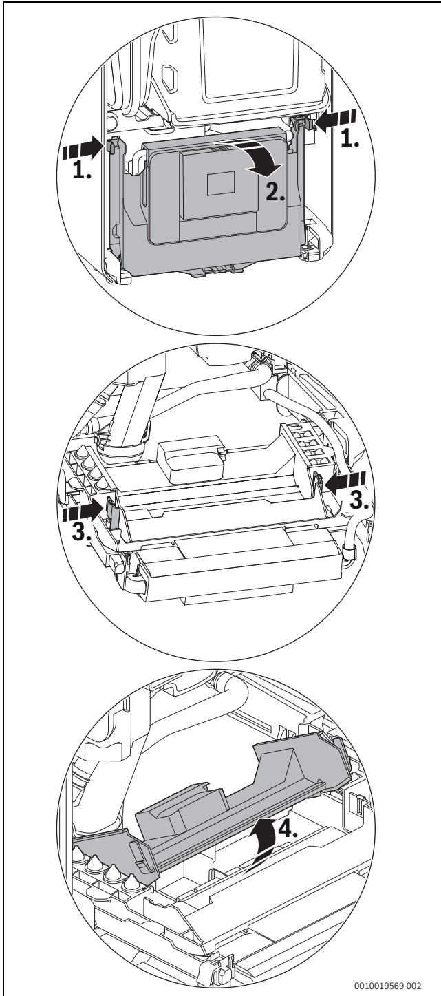
Afb. 80 Afdekking openen
