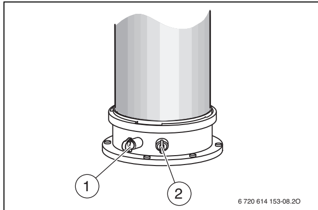
Afb. 105 Rookgasmeetnippel en verbrandingsluchtmeetnippel
