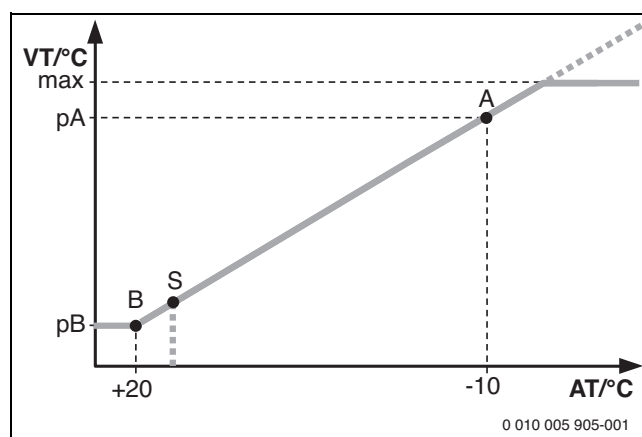
Afb. 81 Stooklijn
