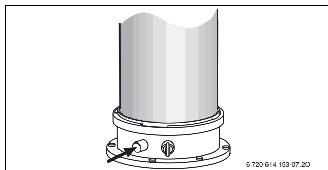
Afb. 37 Rookgasmeetnippel
