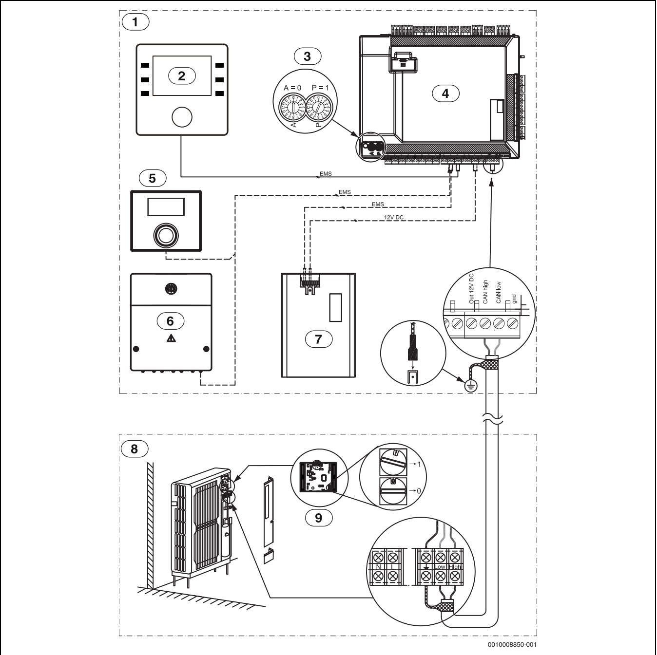
Afb. 31 EMS/CAN-BUS-schakelschema
