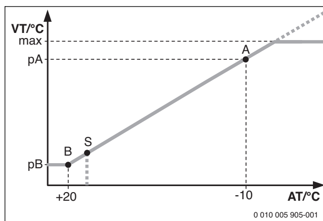
Afb. 78 Stooklijn
