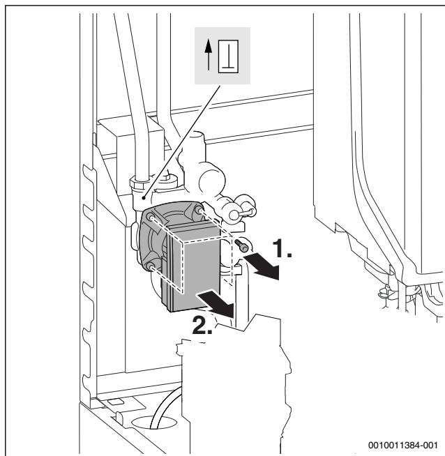
Afb. 110 Demonteer solarpomp
