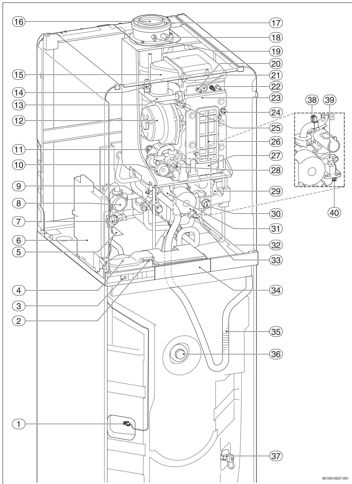
Afb. 17 GC9000iWM 30/150-ketels
