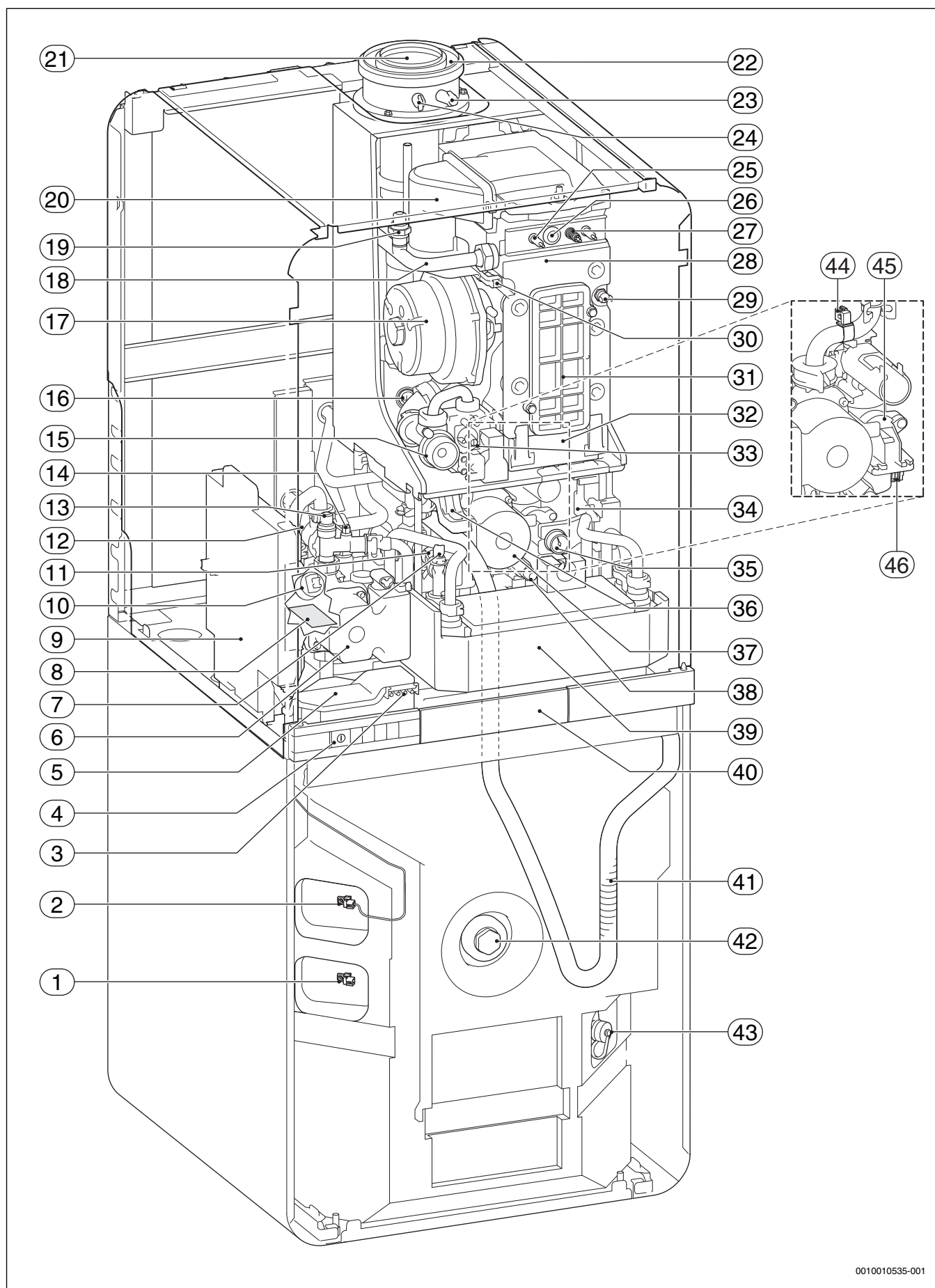
Afb. 18 GC9000iWM.../100..-toestellen
