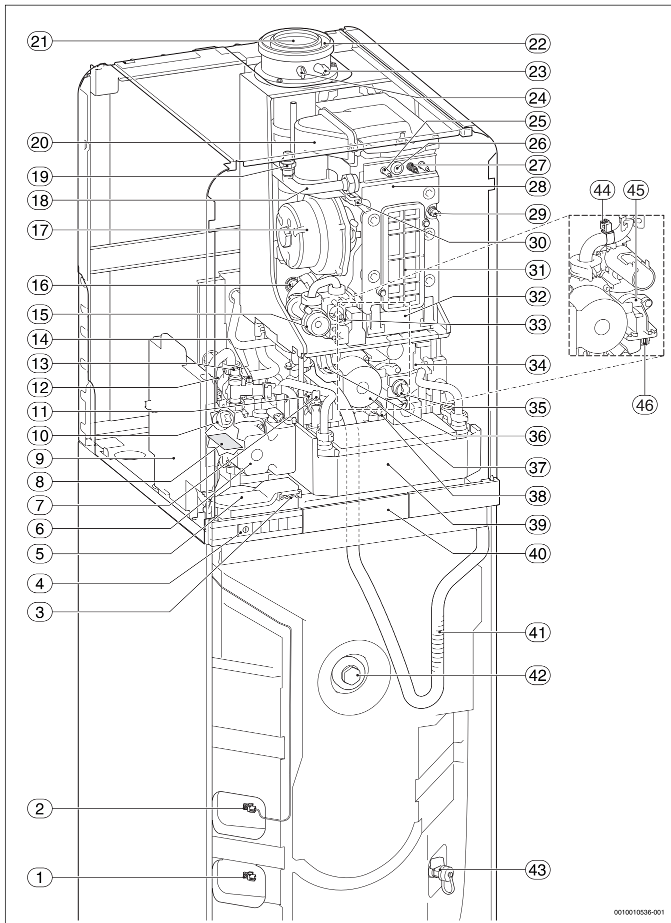
Afb. 17 GC9000iWM.../150..-toestellen
