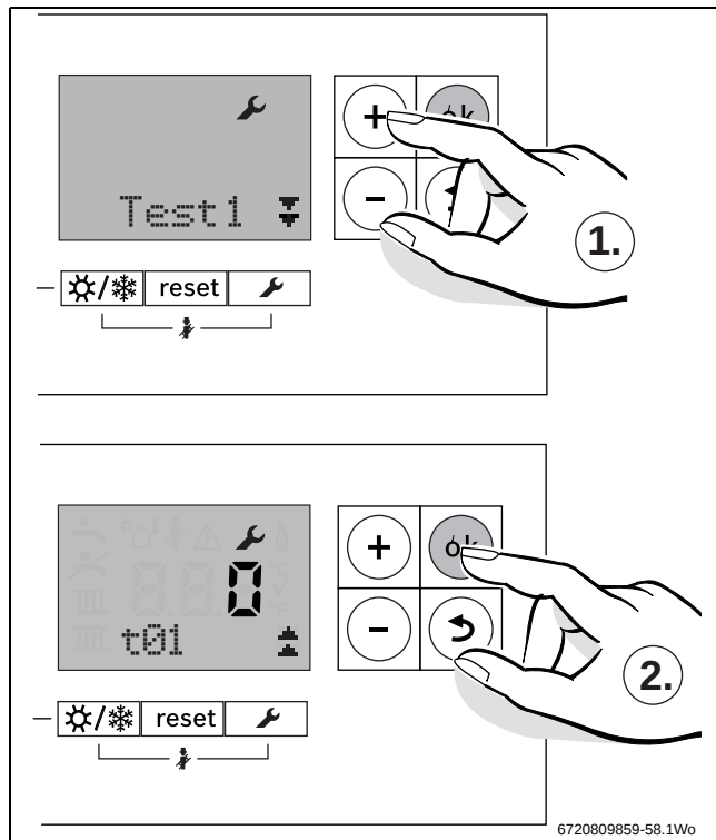
Afb. 75 Selecteer testmenu
