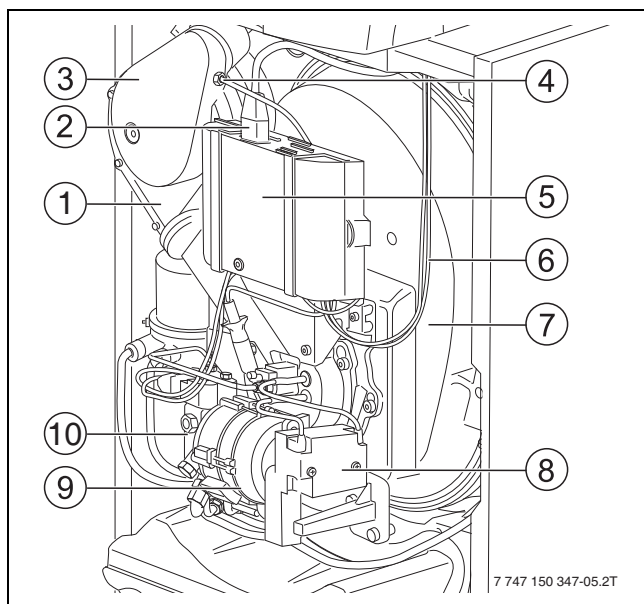
Afb. 2 Stookoliebrander
