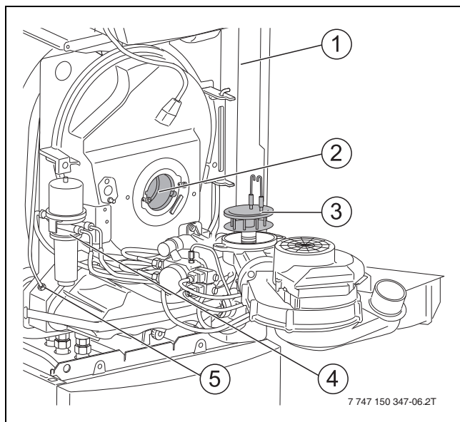
Afb. 3 Stookoliebrander in servicepositie
