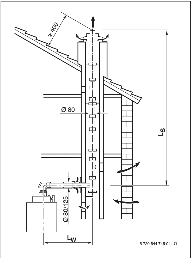
Afb. 11 Parallele buIs in schacht (B 33 , star)
