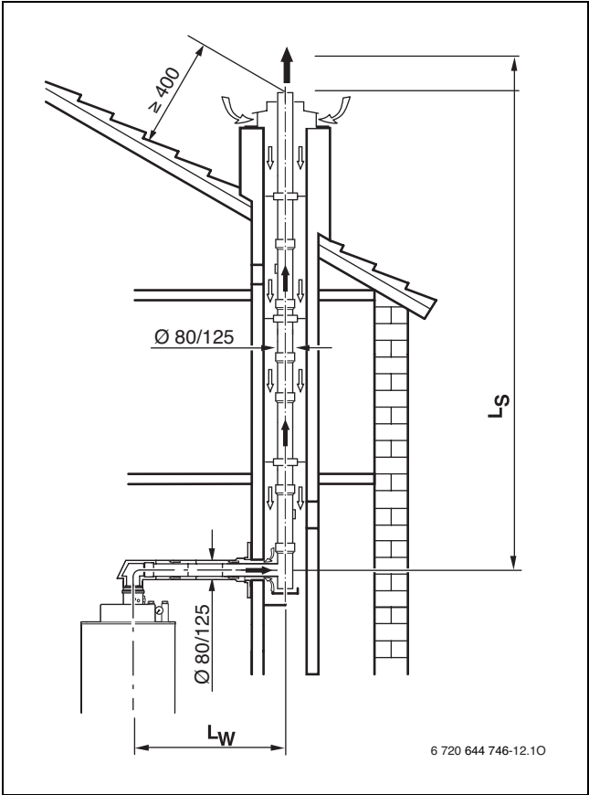
Afb. 19 Rookgasafvoer in schacht ( C_{93(x)} )
