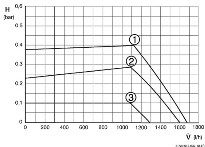
Fig. 66 constante druk TOP 30/475-3 ZBS
