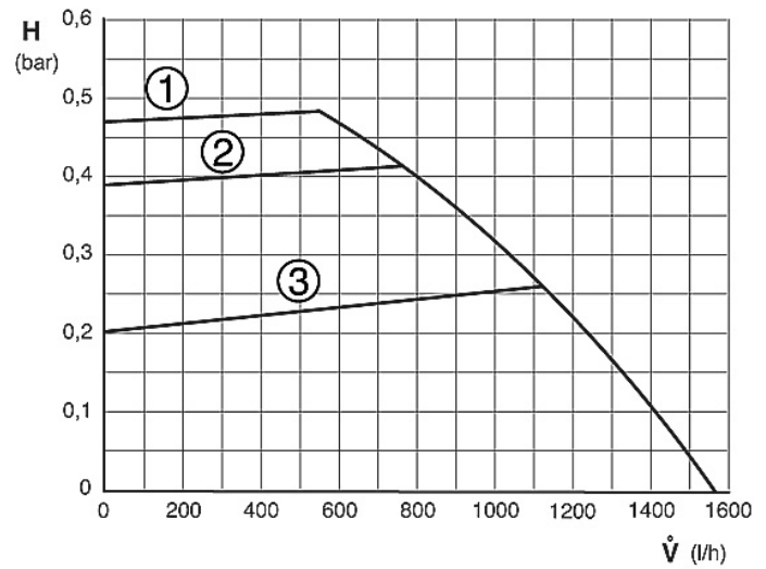
Fig. 65 constante druk TOP 30/475-3 ZBS
