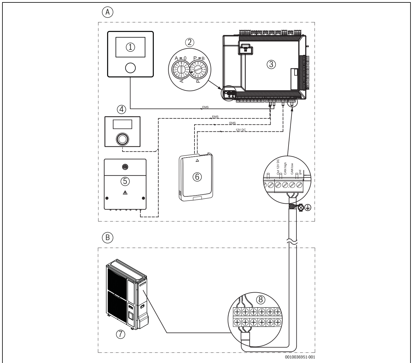
Fig. 39 Raccordements CAN et EMS
