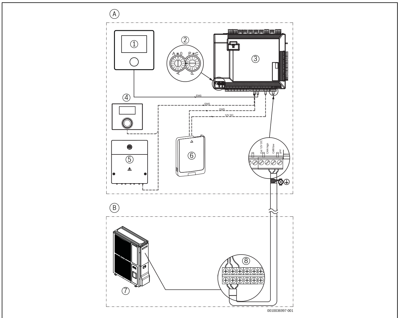
Fig. 41 CAN et raccordements EMS
