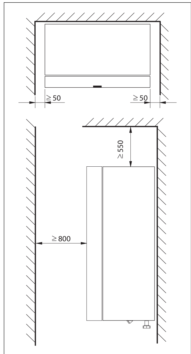
Fig. 3 Distance minimale (mm)
